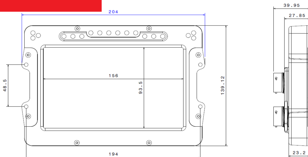
► DASHBOARDS: APPLICATION EXAMPLE NTS 7"
